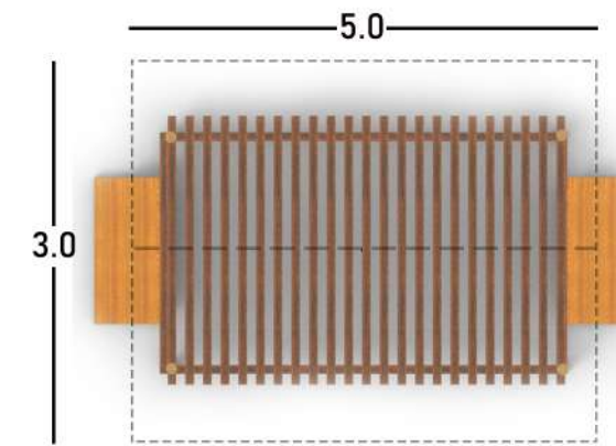
PLAN (1:50)
