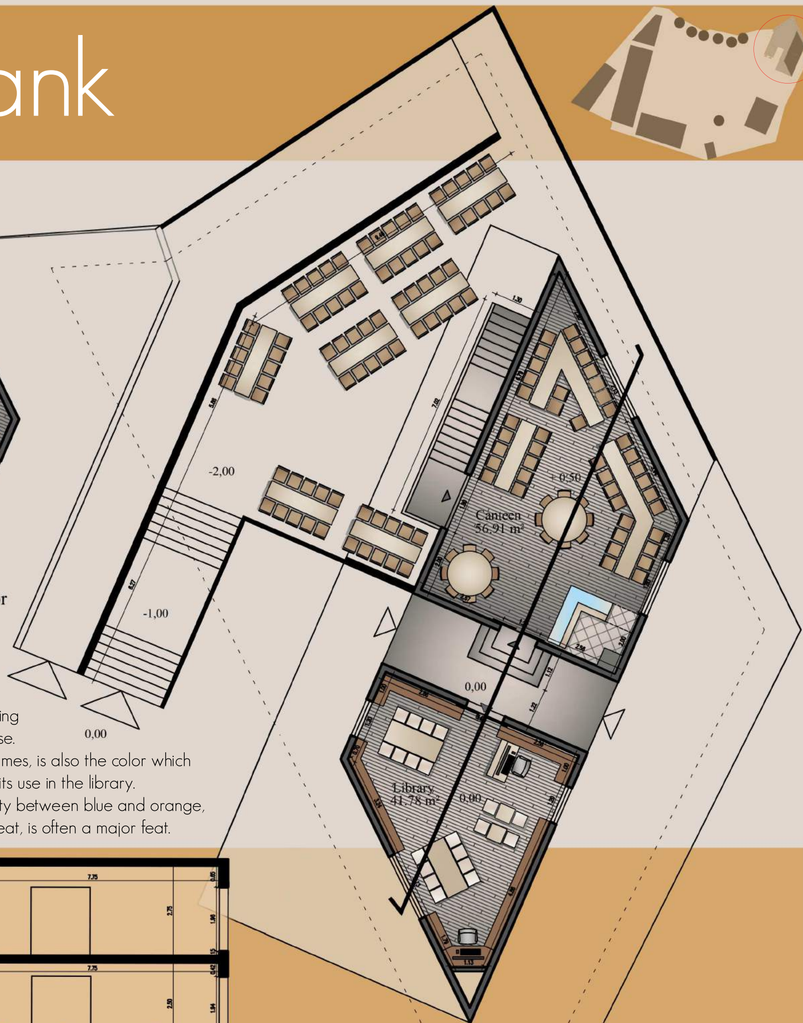
Ground floor
