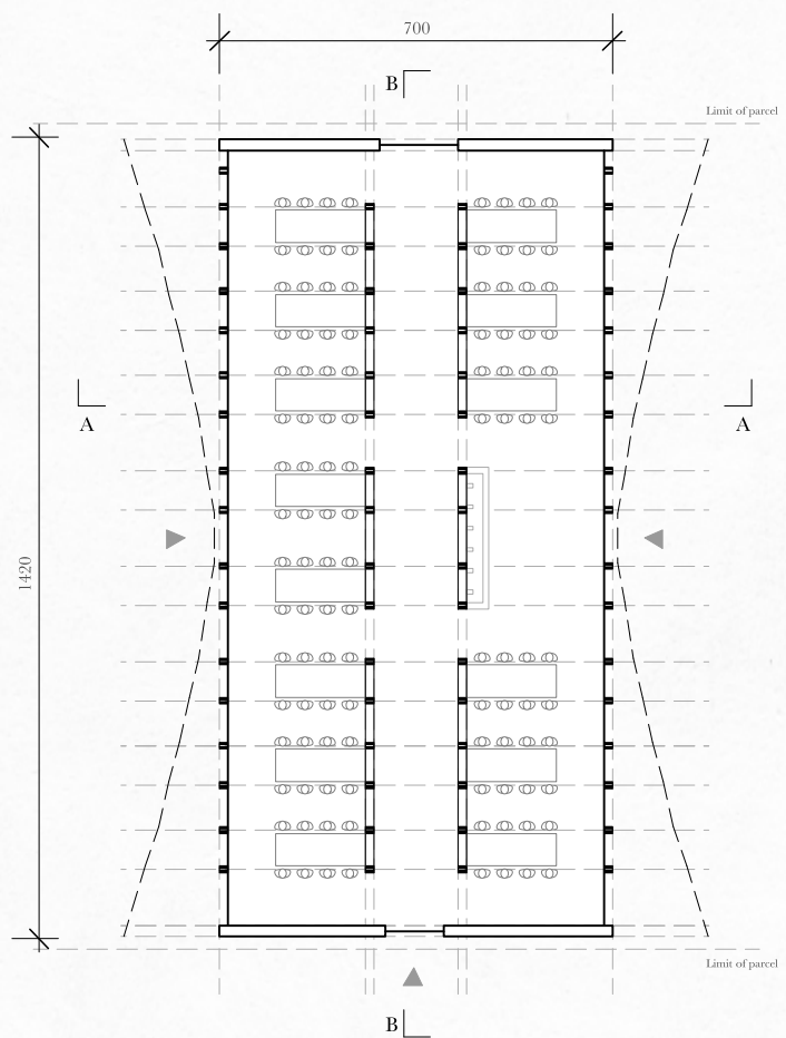
Plan
