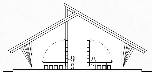
Section a
