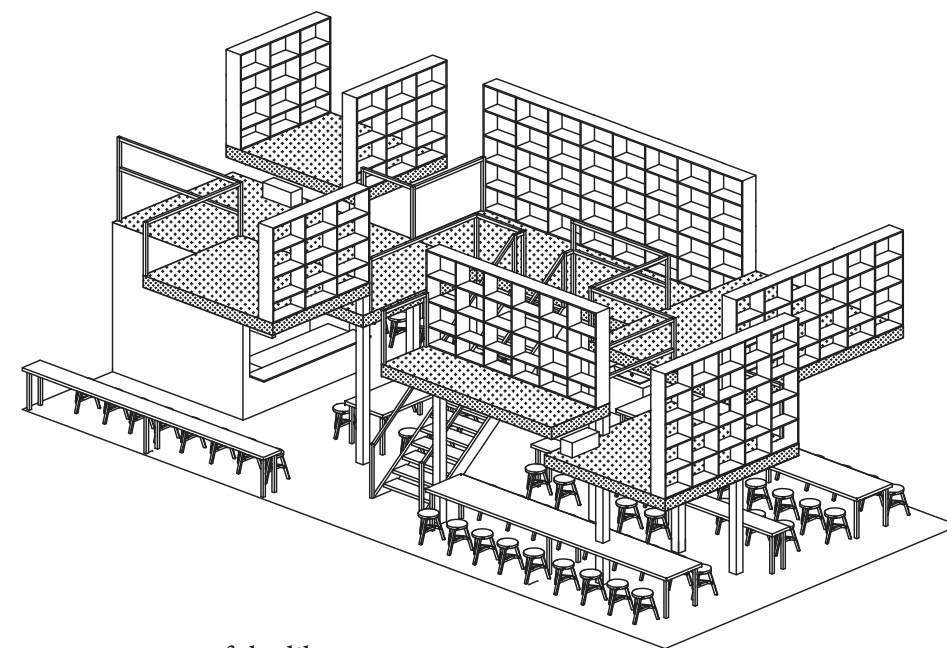
1st floor axonometry of the library
