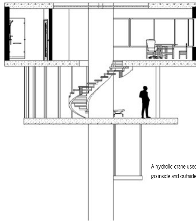
Building Section
